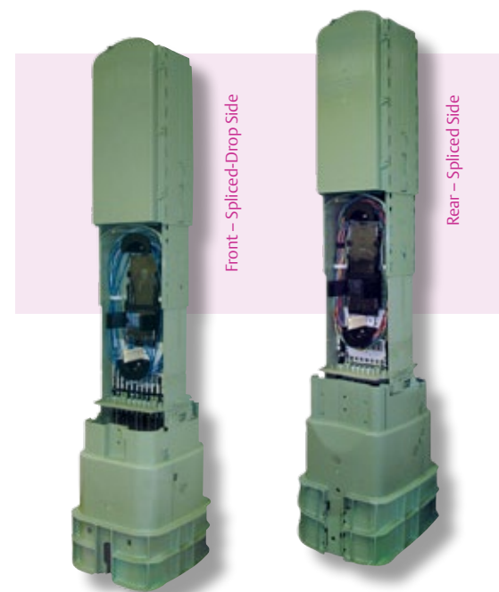
NetSpan FDP Series Integrated Fiber Distribution Pedestal Solution
